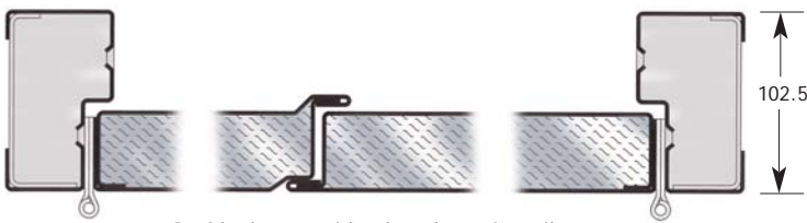
Double doorset with rebated meeting stiles
