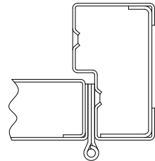
Rebate frame with continuous hinge
