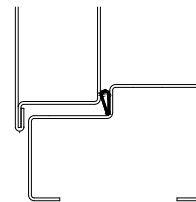
Reverse head threshold Various heights
