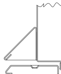
Opening in with weatherboard
